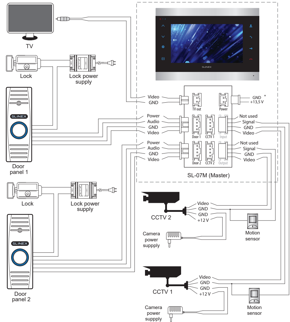
Diagram 1. SL-07M door panels, cameras, locks and TV connection.
