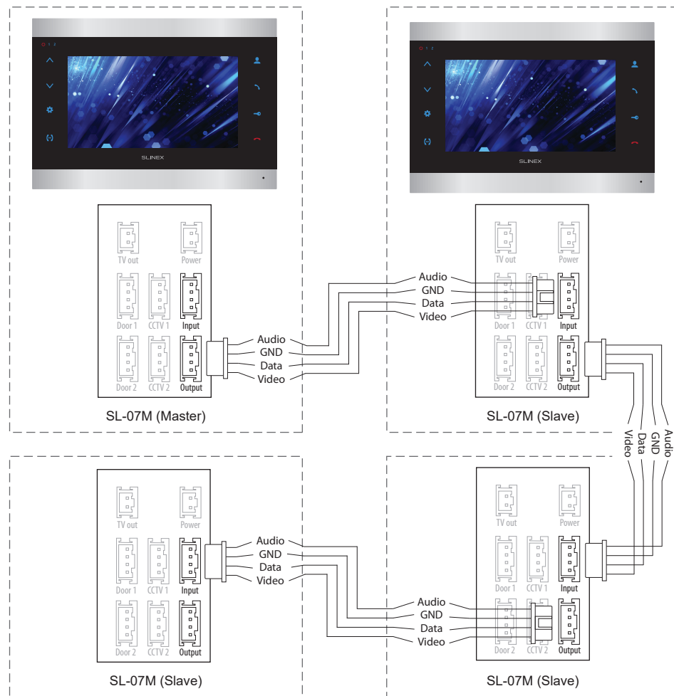
Diagram 2. SL-07M system connection.
