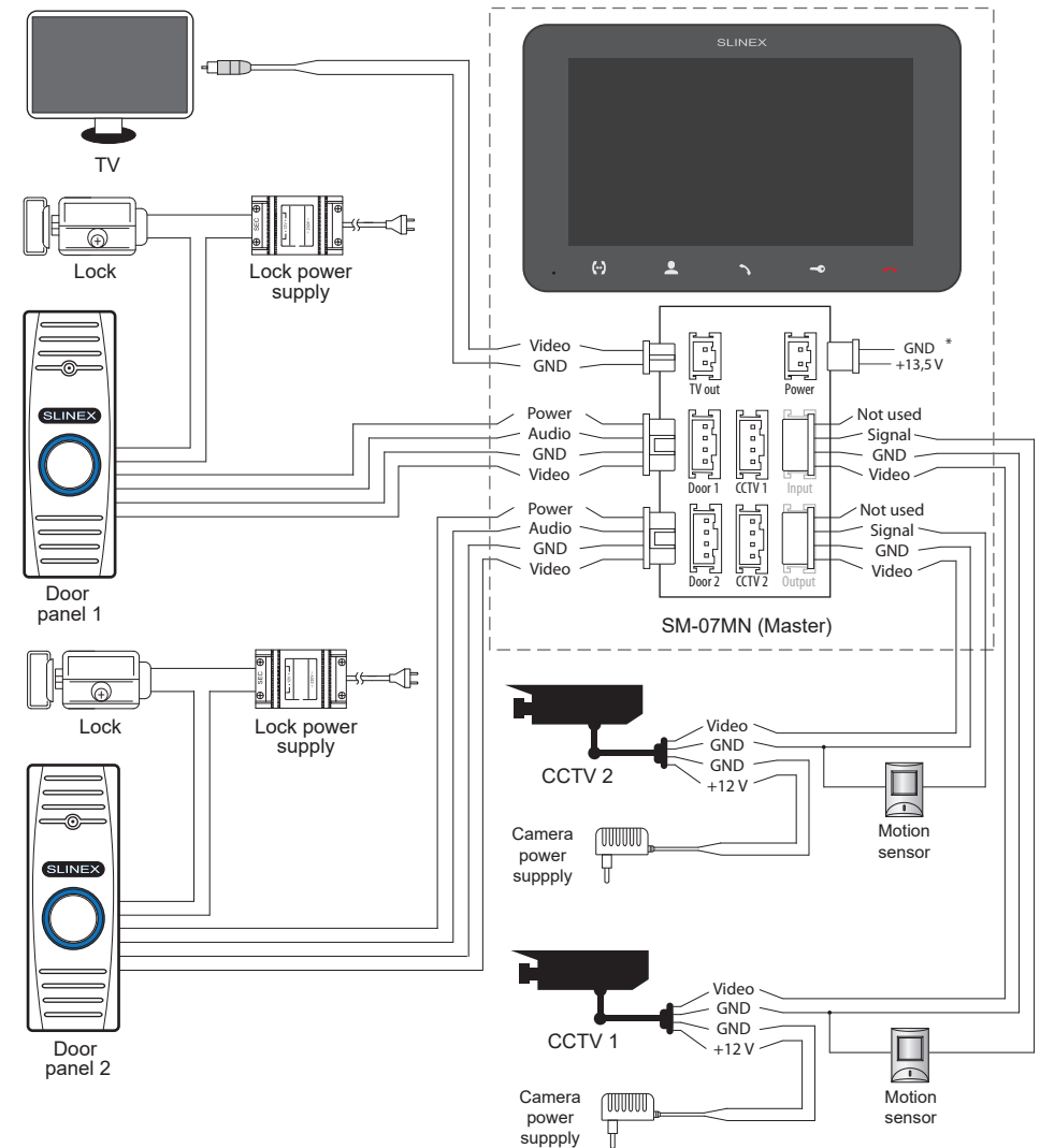
Diagram 1. SM-07MN outdoor panels, cameras and locks connection.
