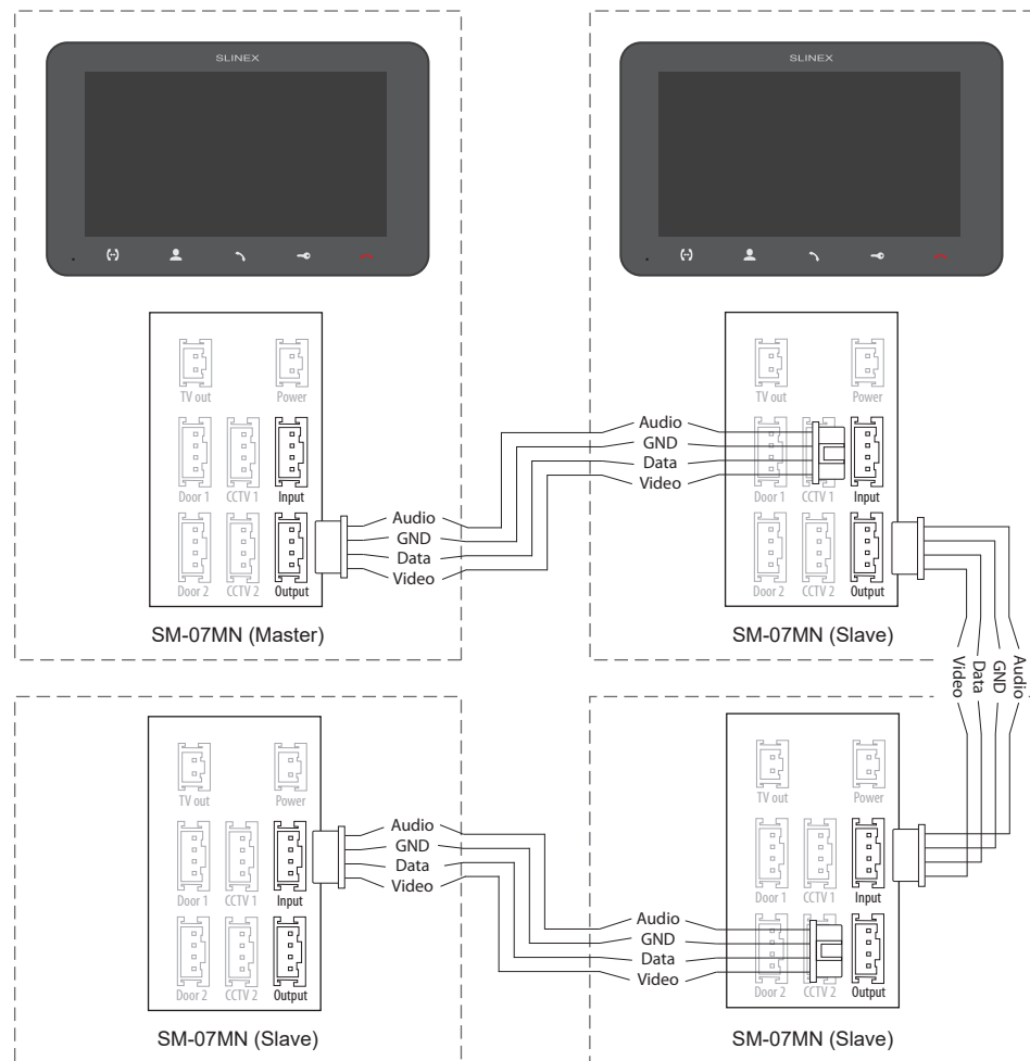
Diagram 2. SM-07MN system connection.
