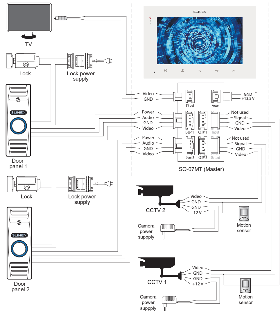
Diagram 1. SQ-07MT door panels, cameras, locks and TV connection.
